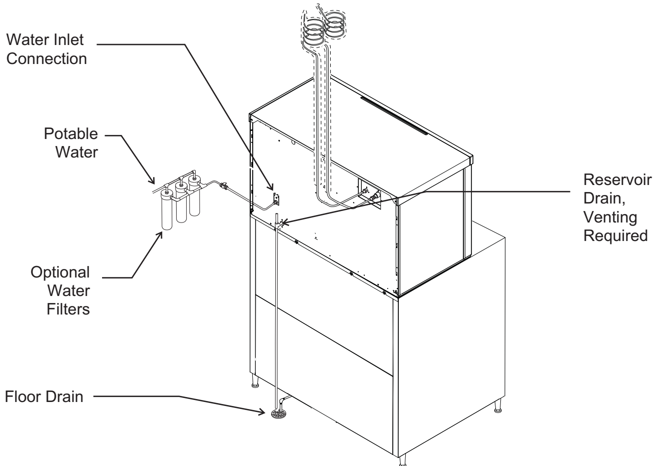
Water Supply and Drain Connections
