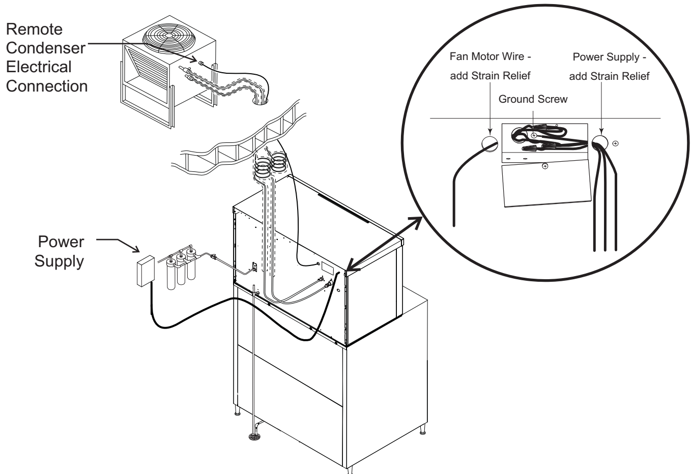
Electrical Connections
