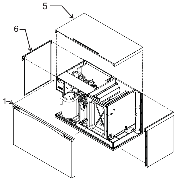
Panel Removal
