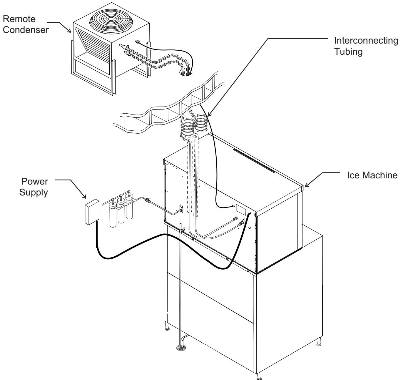
Remote Condenser, Typical System Illustration
