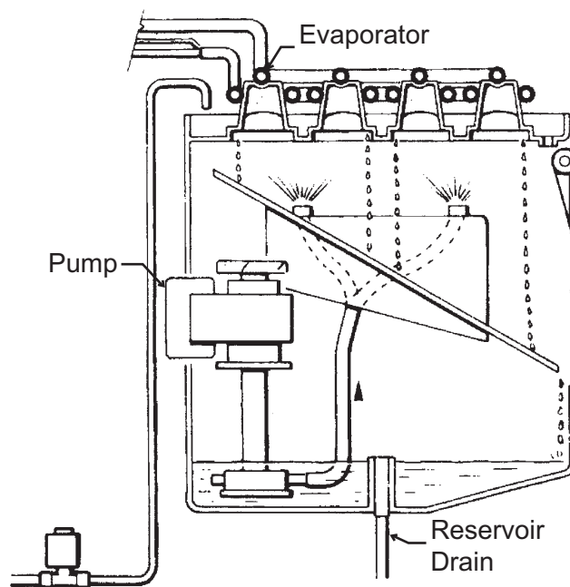
Freeze Cycle Water Schematic
