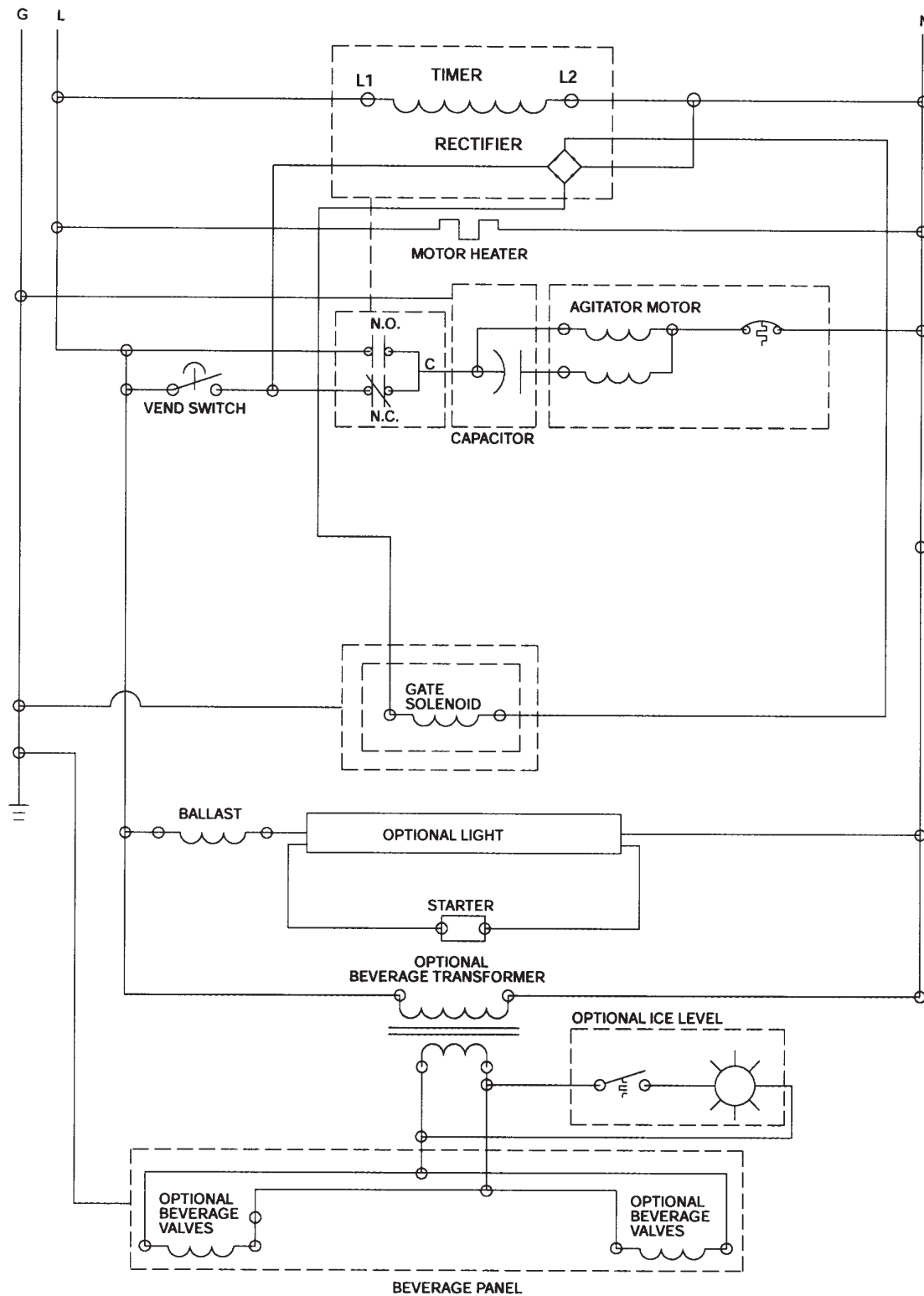
FIGURE 8. WIRING SCHEMATIC (120 V UNIT)
