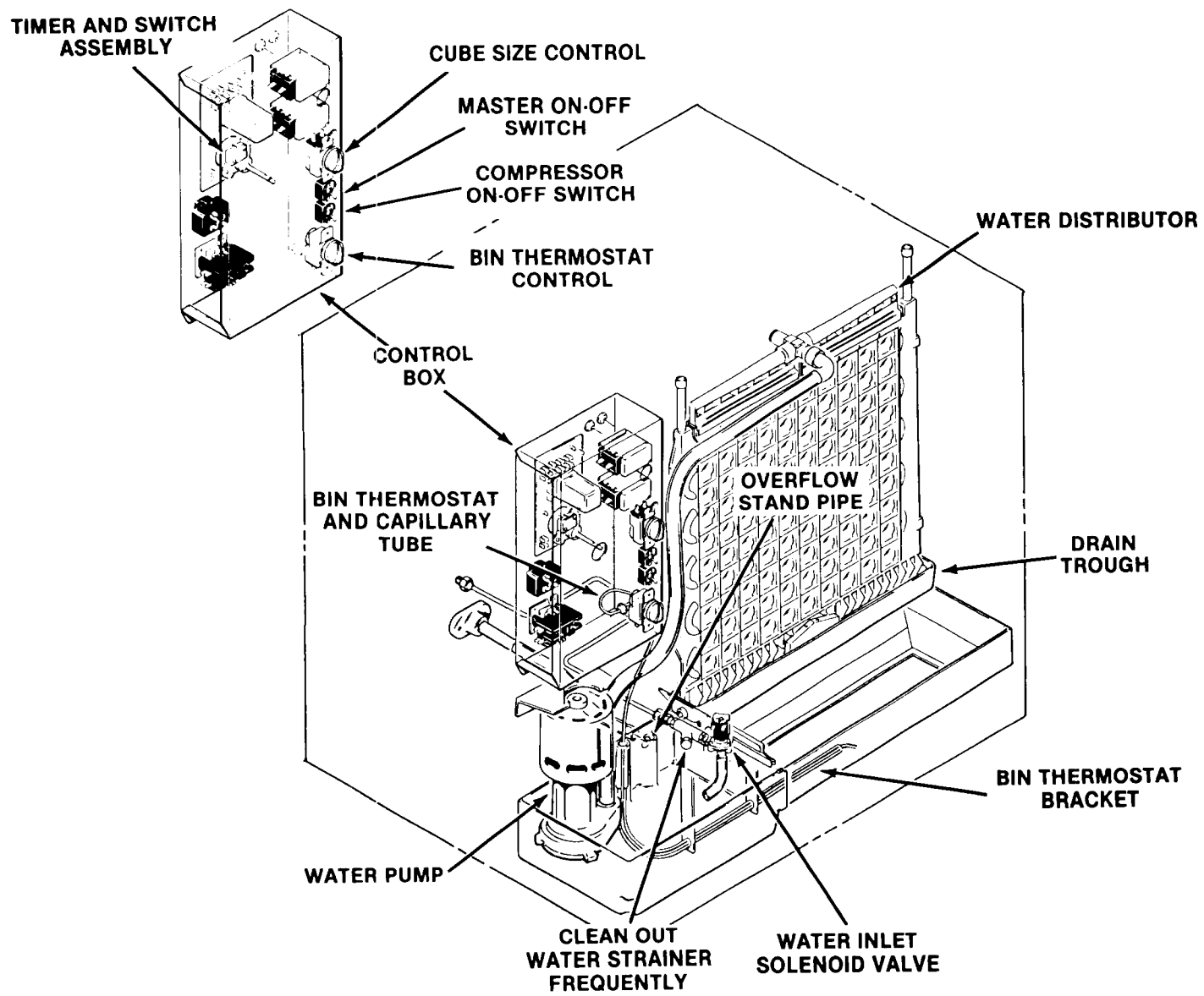
Cleaning Water System, Icemaker
