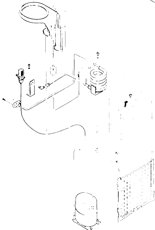
WATER-COOLED ASSEMBLY
