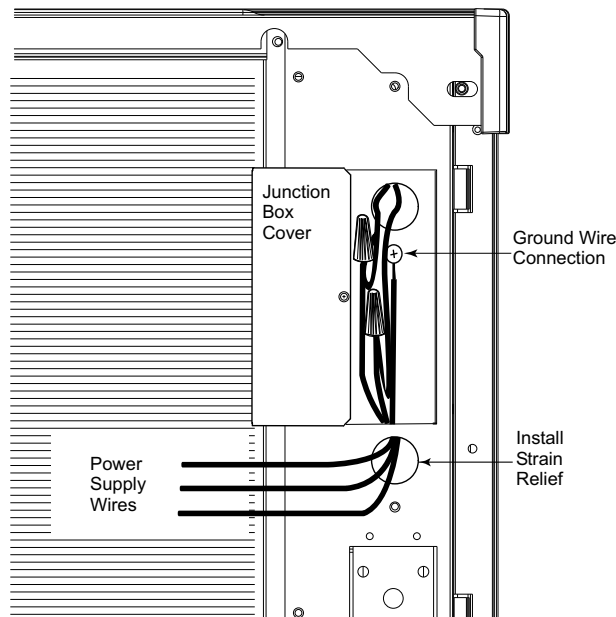
Electrical Connections, Back of Unit
