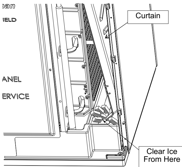
Clear ice From Beneath Curtain
