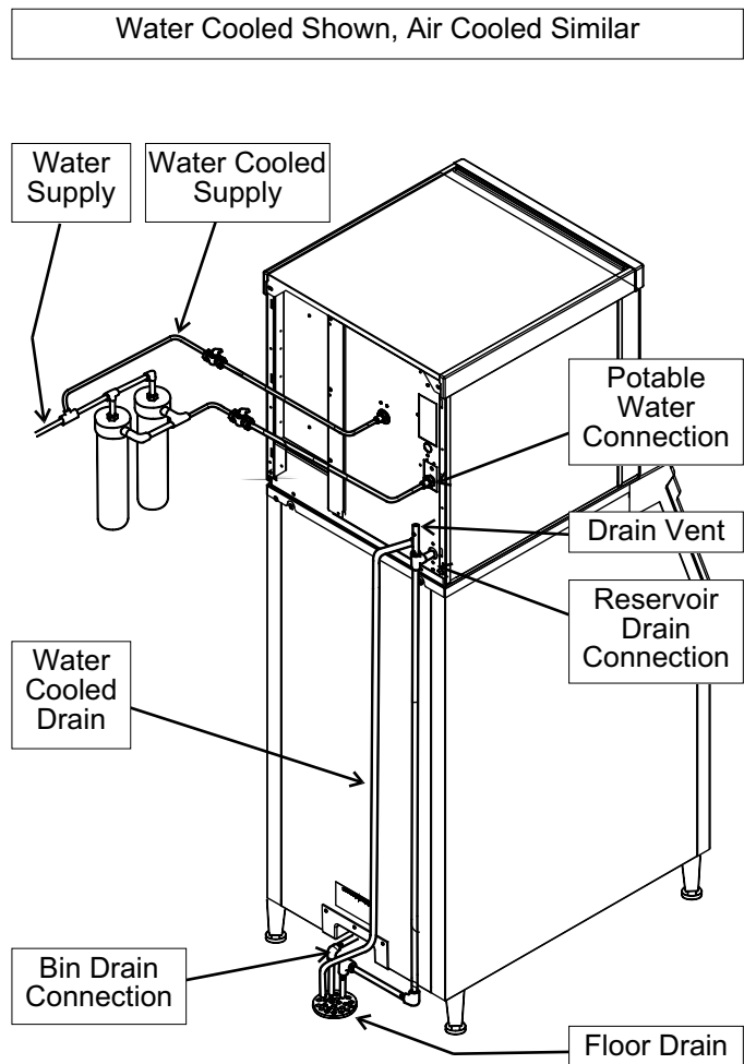
Plumbing Connections
