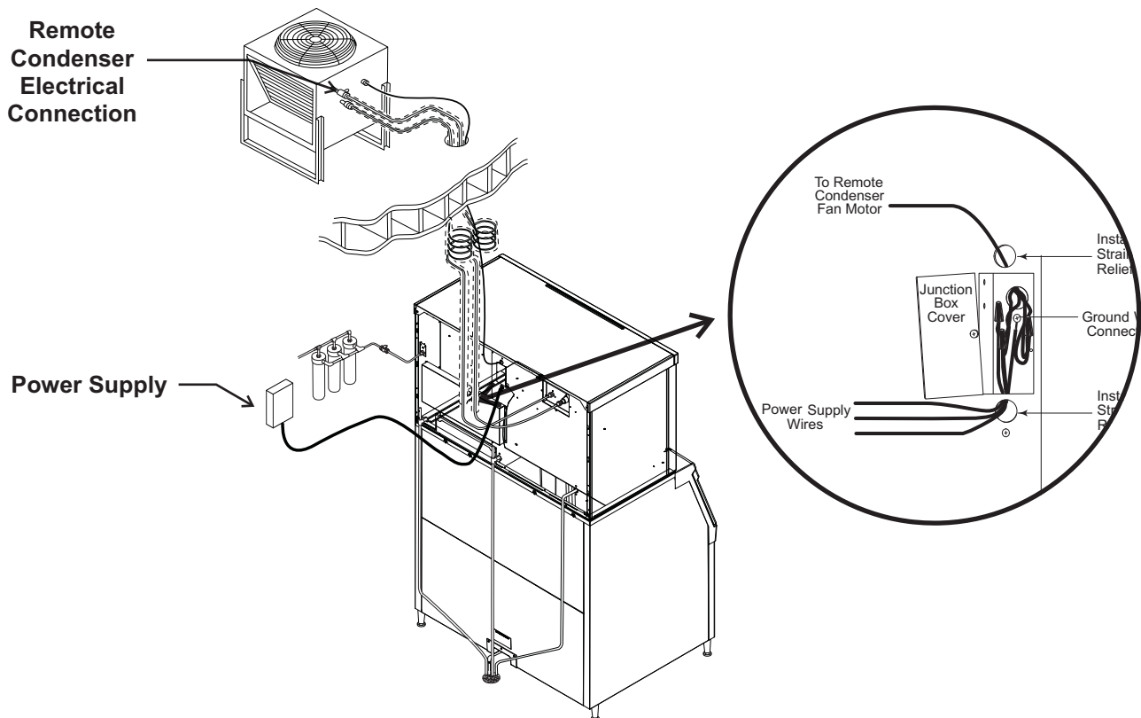
Electrical Connections
